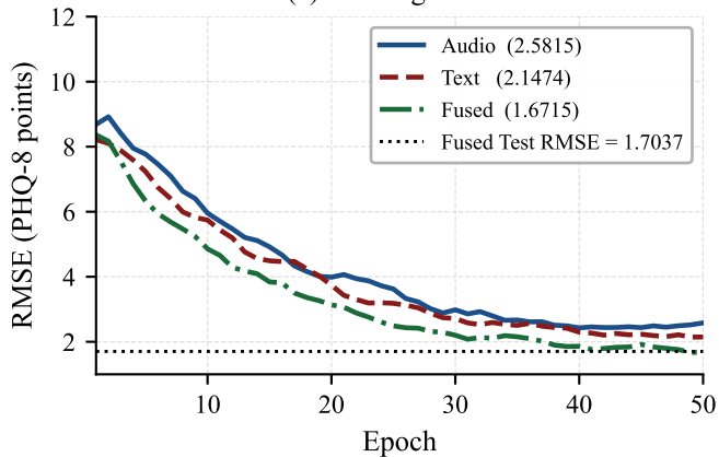
(a) Training RMSE
