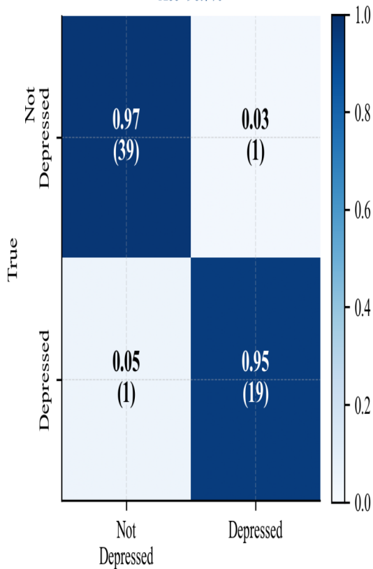
(a) Audio Only Acc=96.7%
