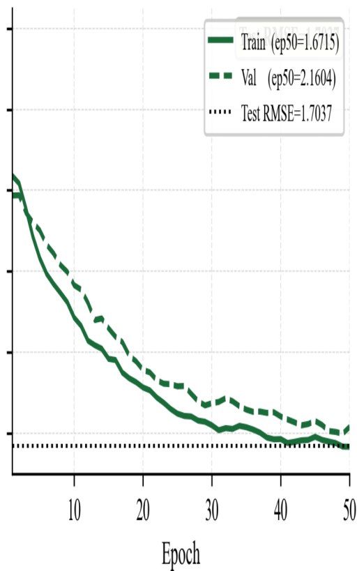
Fused (Audio + Text) (DG-HMCF)
