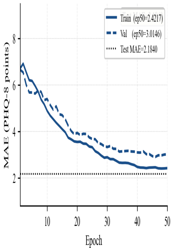
Audio Only (Way2Vec2 + BiLSTM)
