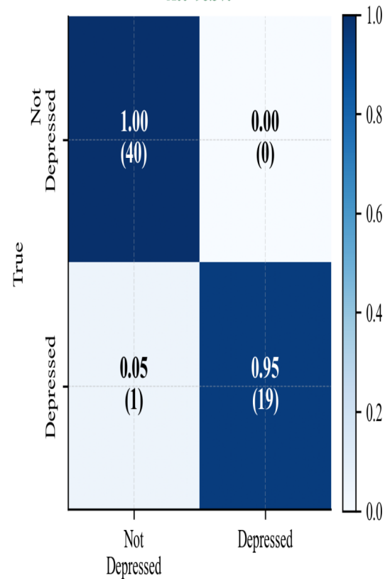
(c) Fused (Audio+Text) Acc=98.3%
