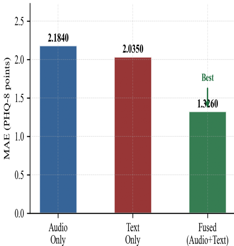
(a) Mean Absolute Error (MAE)
