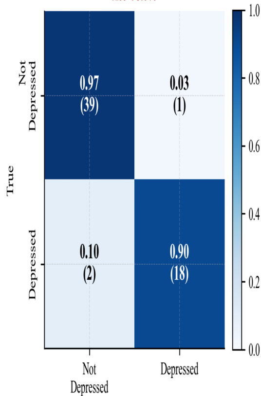
(b) Text Only Acc=95.0%
