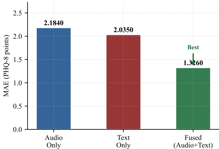
(a) Mean Absolute Error (MAE)
