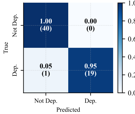
(c3) Fused Confusion Matrix Acc=98.3% F1=0.974
