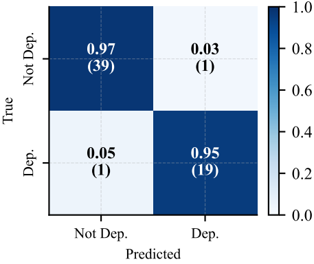
(c1) Audio Confusion Matrix Acc=96.7% F1=0.950
