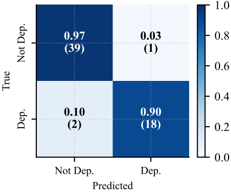
(c2) Text Confusion Matrix Acc=95.0% F1=0.923
