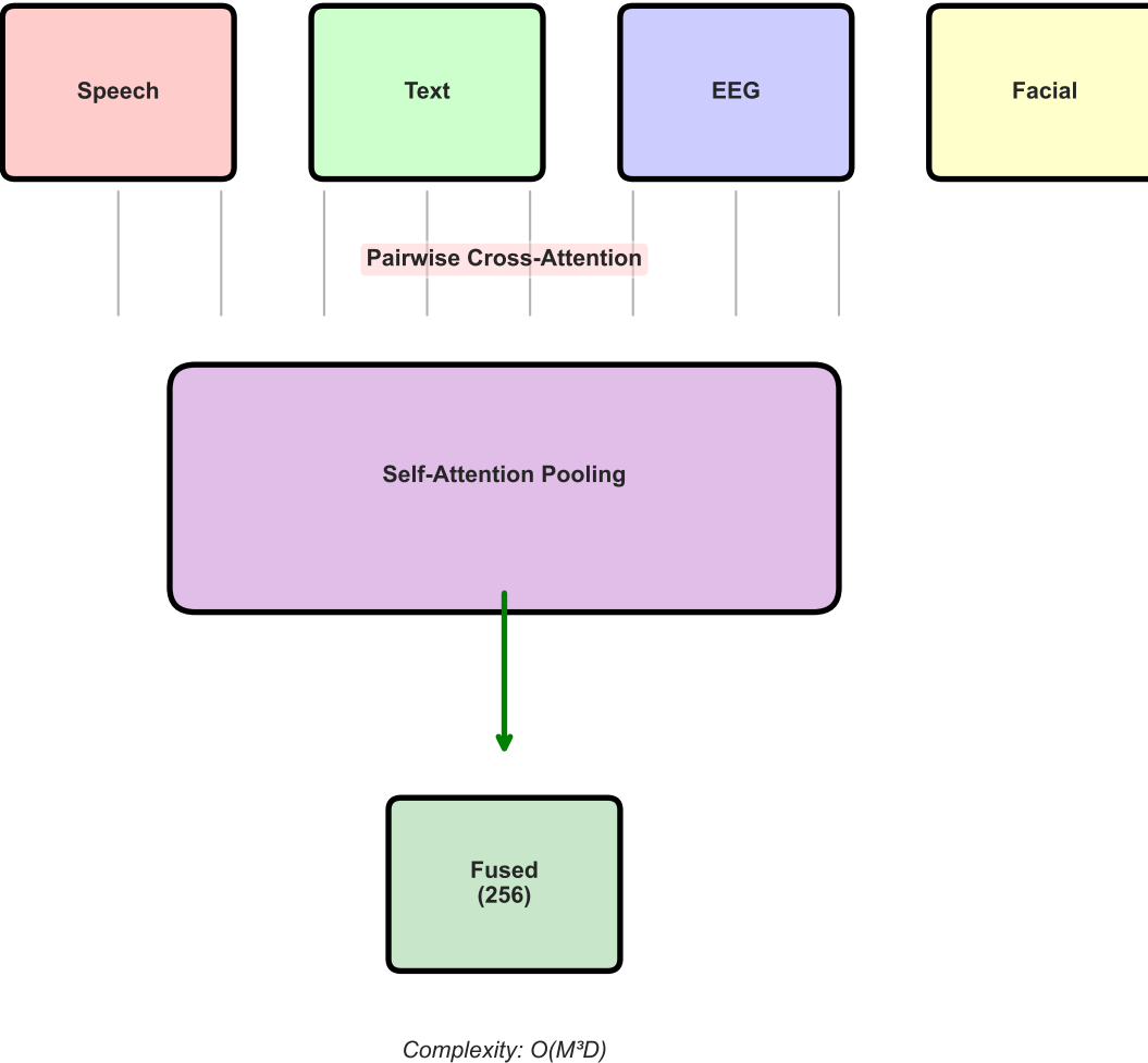
Cross-Modal Fusion (Pairwise Attention)
