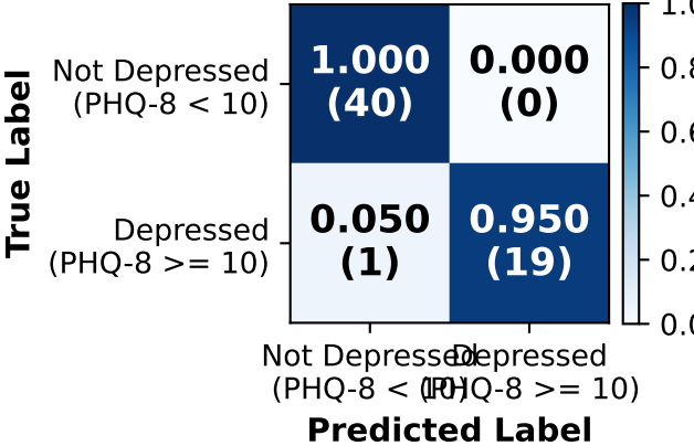
Test Set — Normalized Sensitivity=0.950 Specificity=1.000
