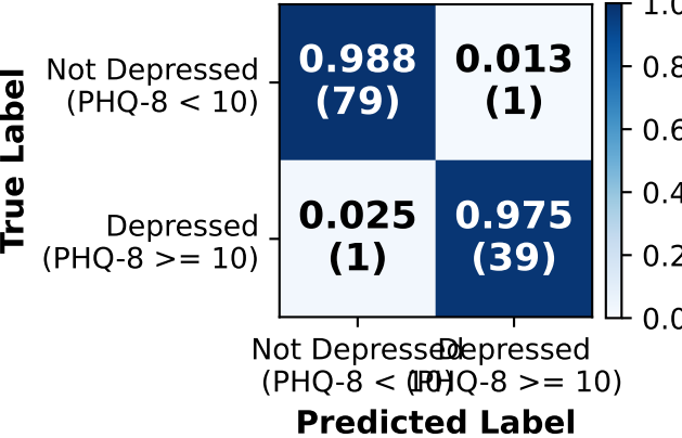
Validation Set — Normalized Sensitivity=0.975 Specificity=0.988
