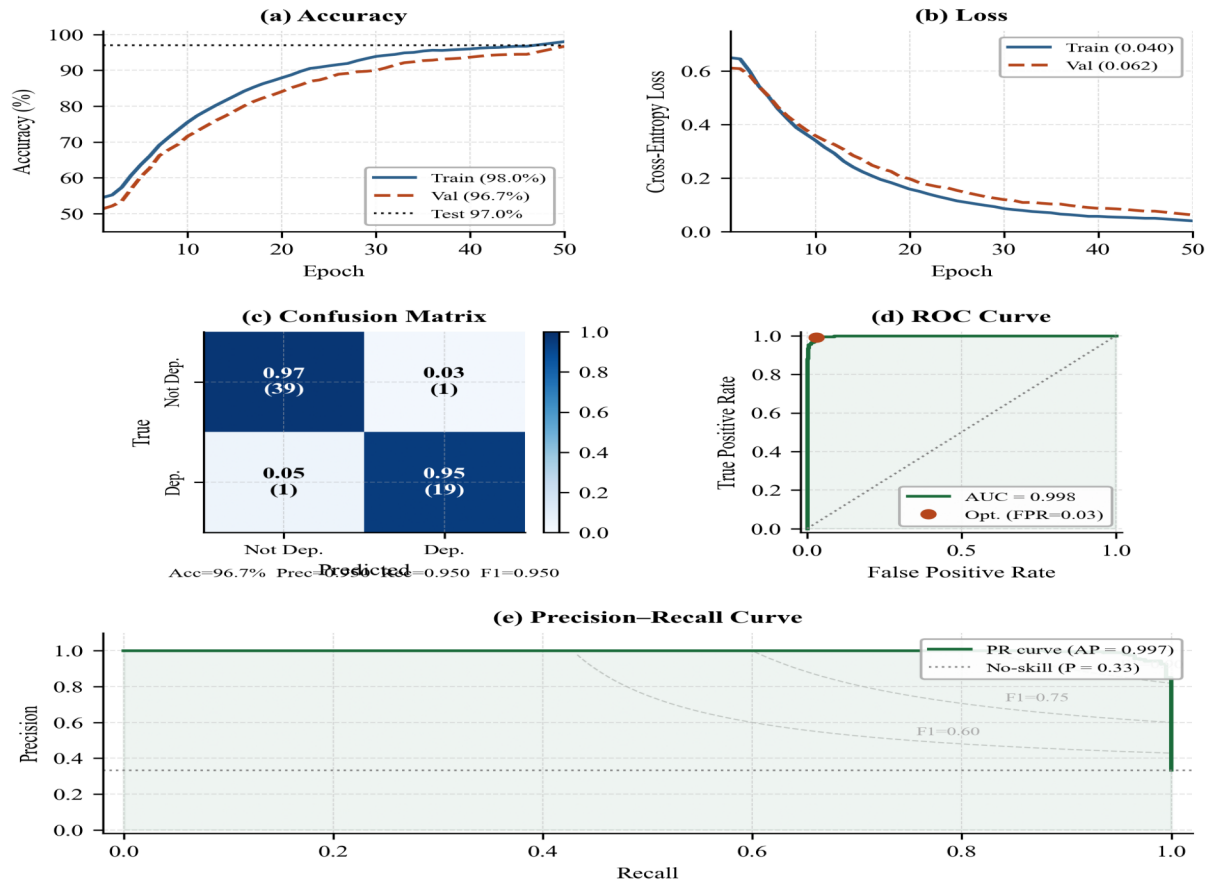
Fig. 1. Evaluation results for the Wav2Vec2 + BiLSTM speech-only depression detection model on DAIC-WOZ. Test accuracy: 97.0%. ROC-AUC: 0.998. AP: 0.997.
