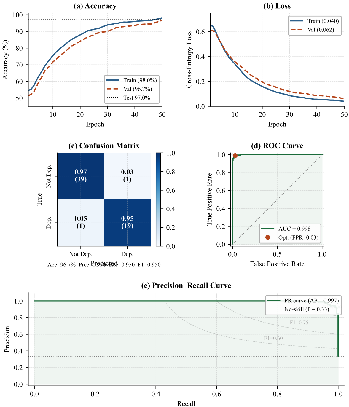
Fig. 1. Evaluation results for the Wav2Vec2 + BiLSTM speech-only depression detection model on DAIC-WOZ. Test accuracy: 97.0%. ROC-AUC: 0.998. AP: 0.997.
