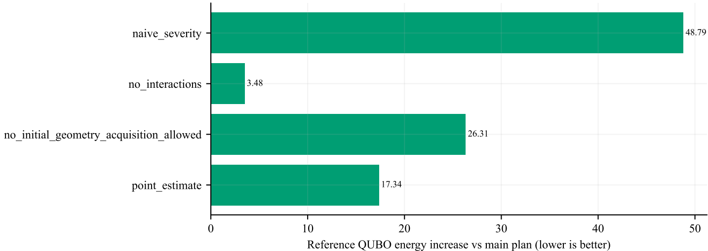
Ablations scored under the same uncertainty-aware objective
