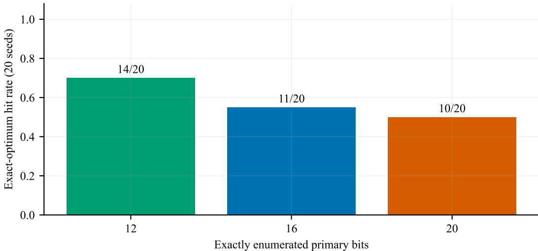
Annealer verification degrades as exact instances grow
