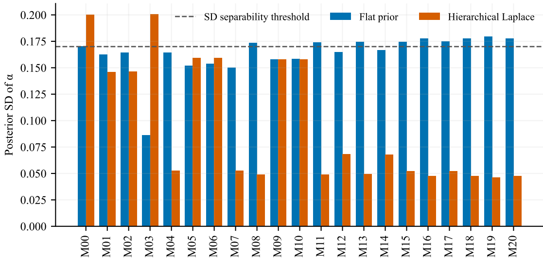
Per-member uncertainty: flat versus sparse prior
