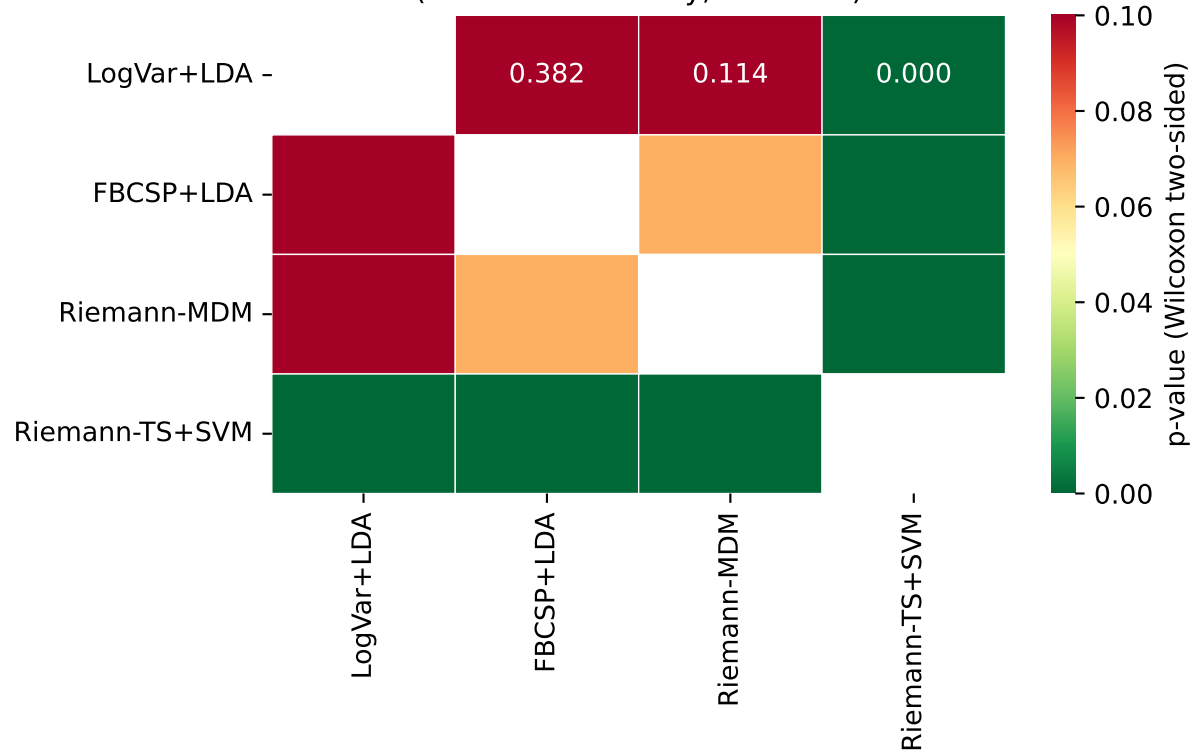
Statistical Significance (balanced accuracy, Wilcoxon)
