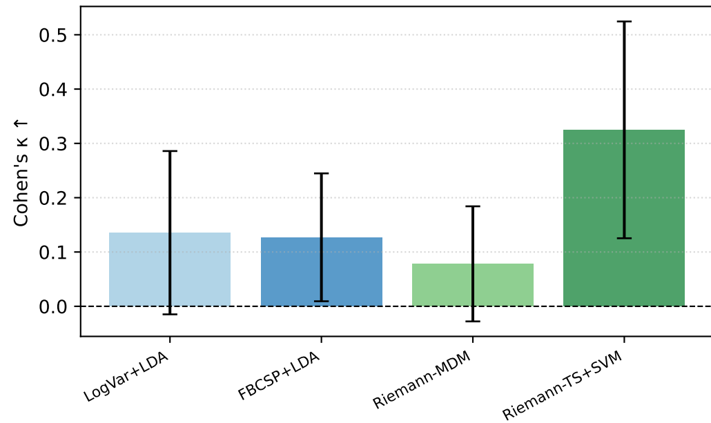
Cohen's Kappa (LOSO)
