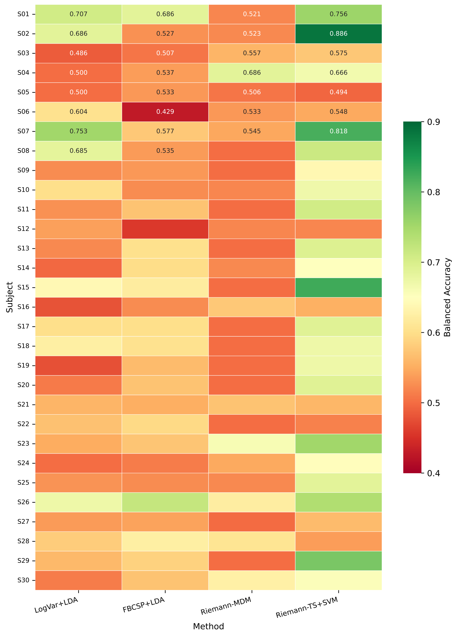
Per-Subject Balanced Accuracy — LOSO (30 subjects × 4 methods)
