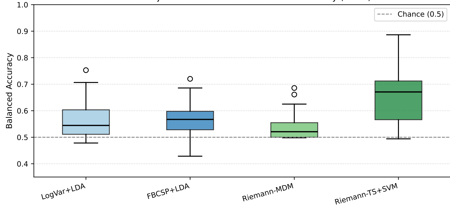
Cross-Subject MI Classification: Balanced Accuracy (LOSO)
