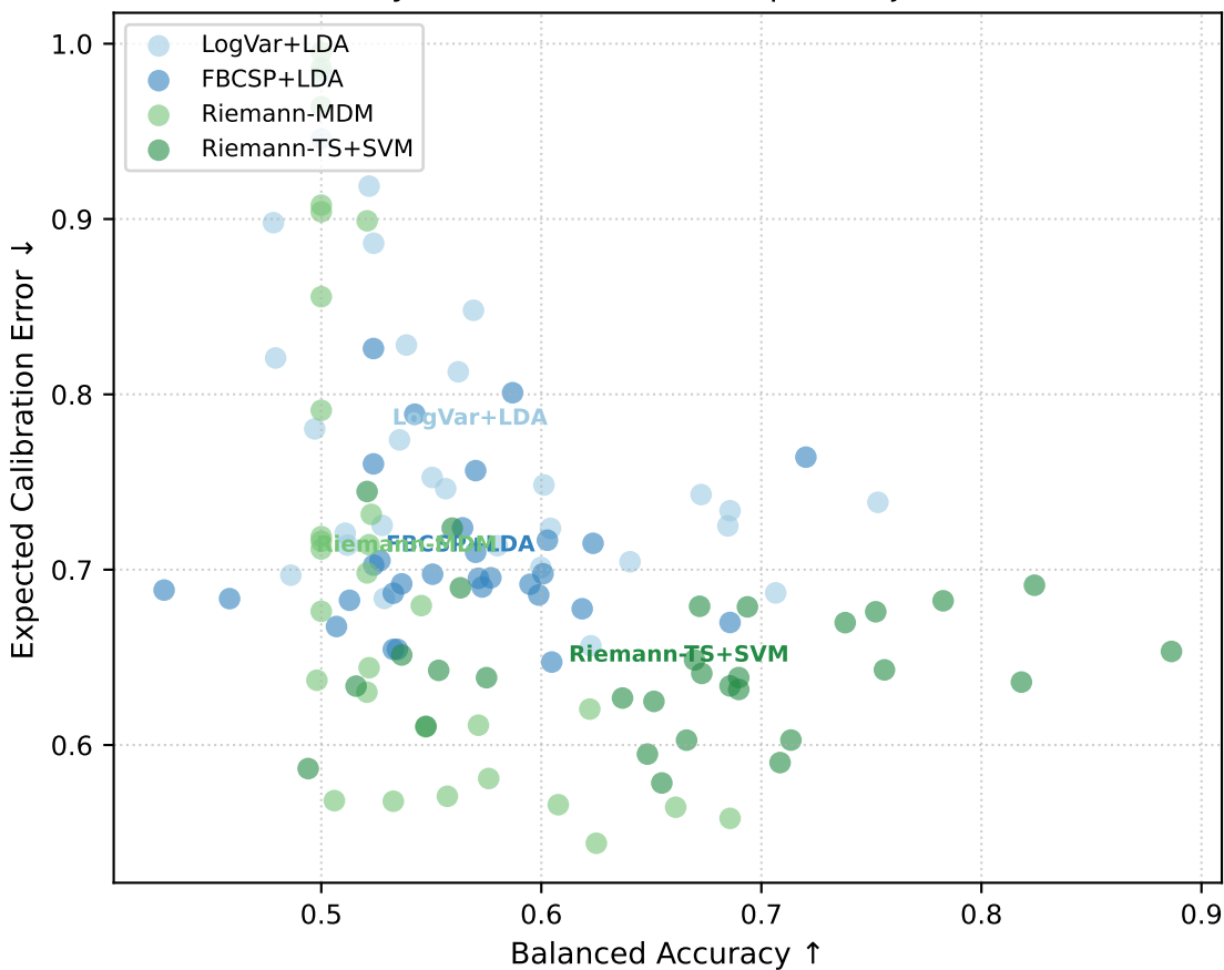
Accuracy-Calibration Tradeoff (per subject, LOSO)
