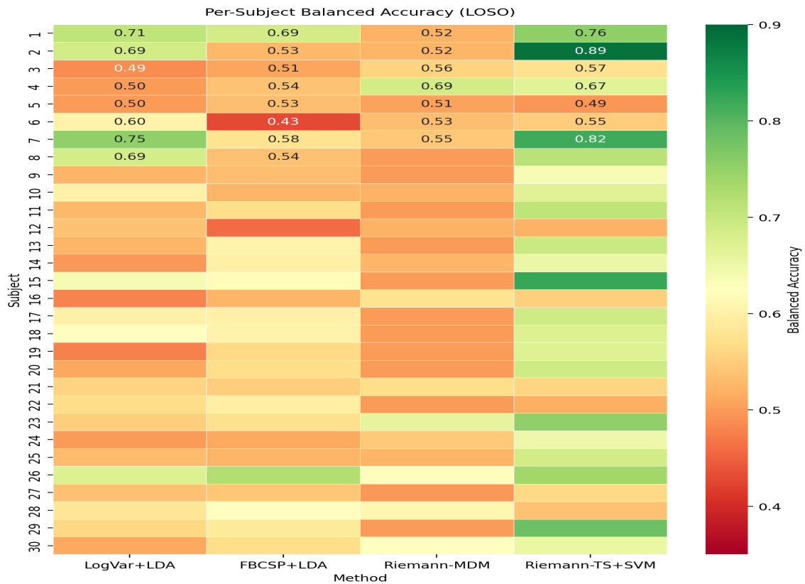
Fig. 2. Heatmap of per-subject balanced accuracy (30 subjects \times 4 methods). Green = high accuracy, red = low. The rightmost column (Riemann-TS+SVM) shows the most green cells. Subject difficulty is correlated across methods (Pearson r \approx 0.61 for LogVar+LDA vs. TS+SVM), suggesting subject-level signal quality is the dominant factor for low-performing subjects.
