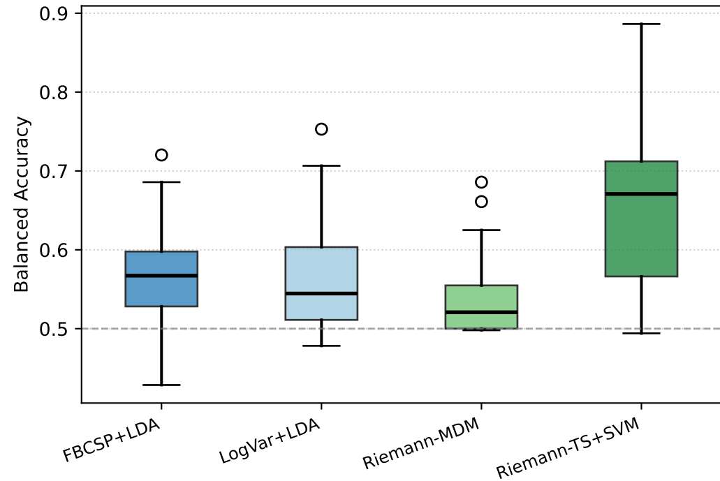
Cross-Subject MI Performance (LOSO)
