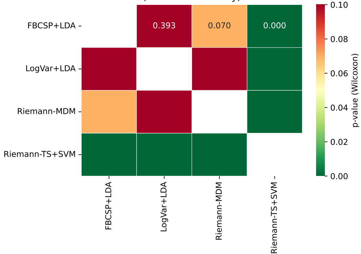
Wilcoxon Signed-Rank p-values (balanced accuracy)
