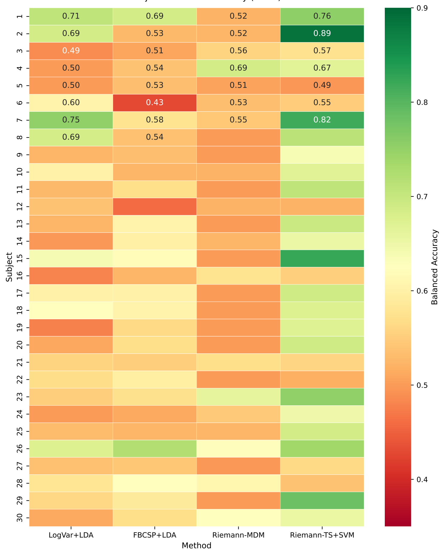
Per-Subject Balanced Accuracy (LOSO)
