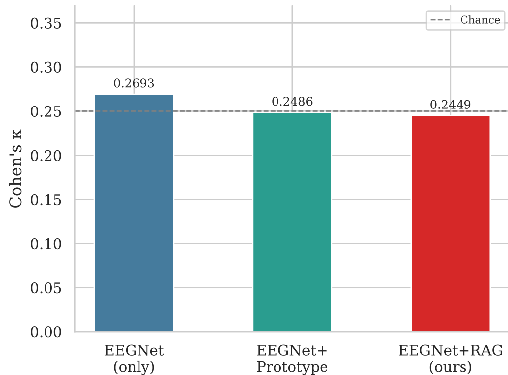
EEGNet + RAG vs. Baselines — PhysioNet EEGMMIDB (Subject-Independent)
