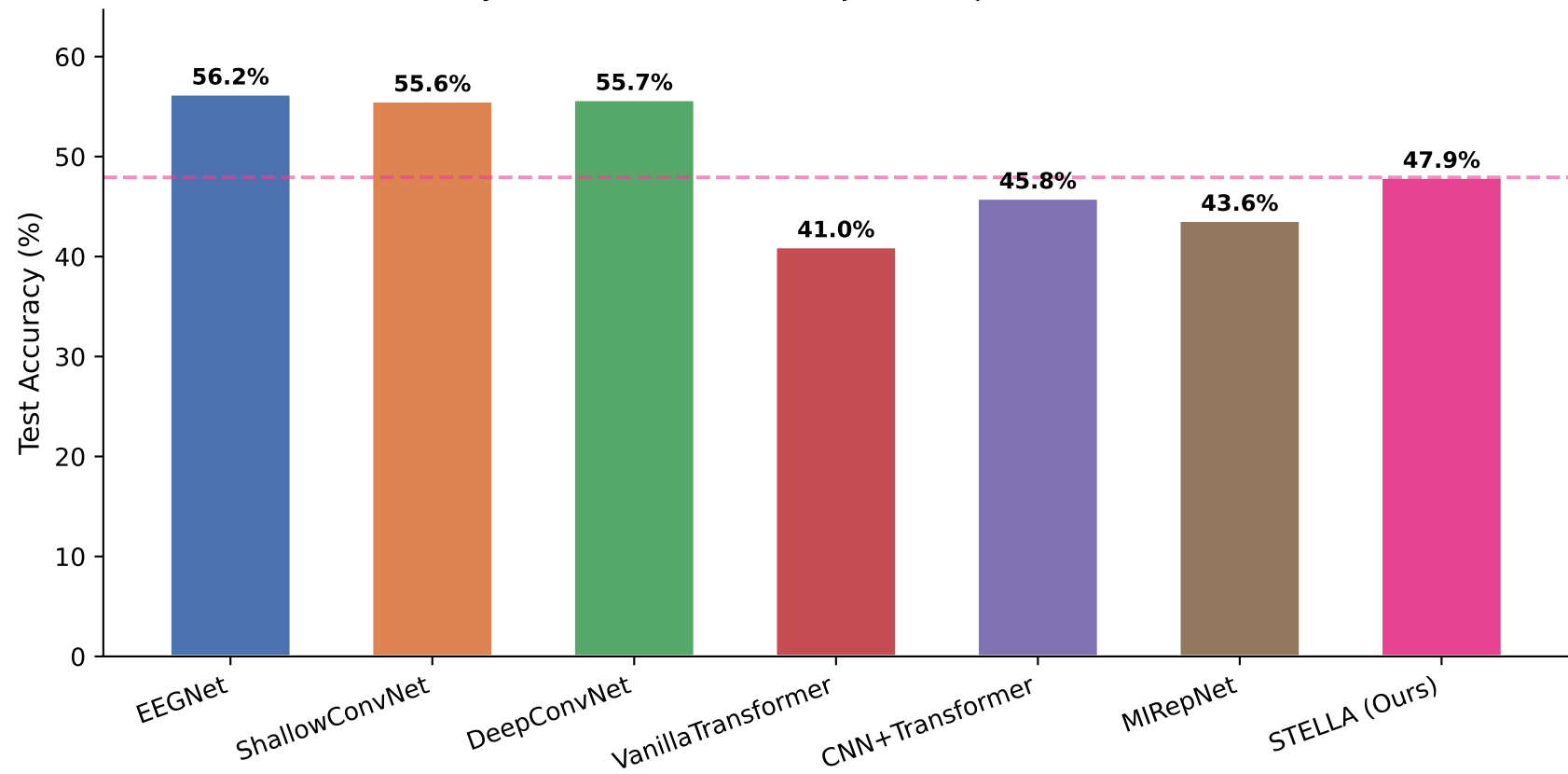
Figure 1: Motor Imagery Classification — STELLA vs. Baselines (PhysioNet EEGMMIDB, Subject-Independent Protocol)
