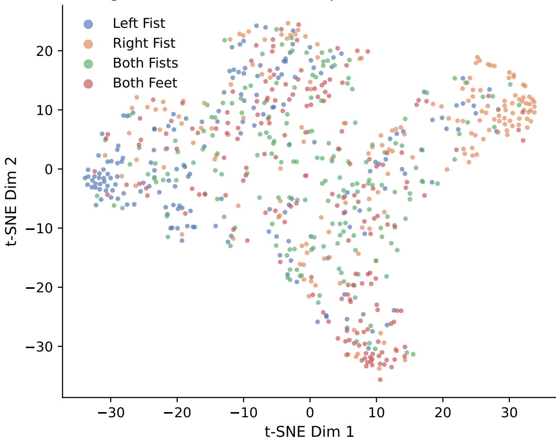
Figure 4: t-SNE of STELLA Representations (Test Set)
