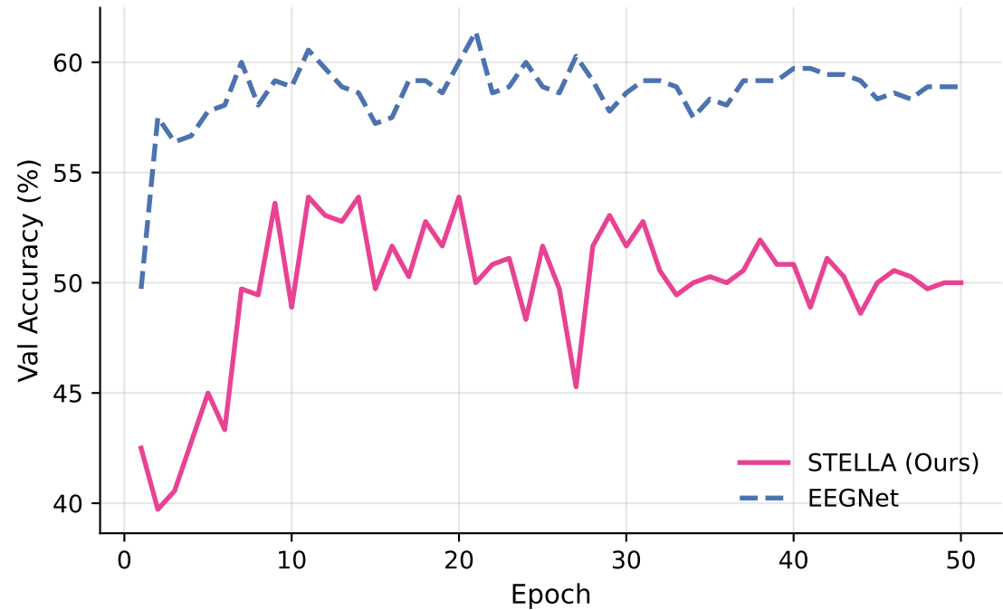
Figure 5b: Fine-tuning Validation Accuracy
