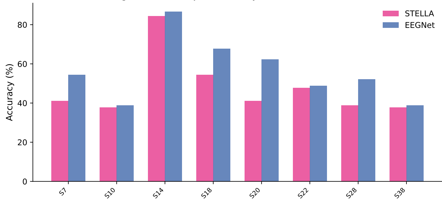
Figure 6: Per-Subject Accuracy — STELLA vs EEGNet
