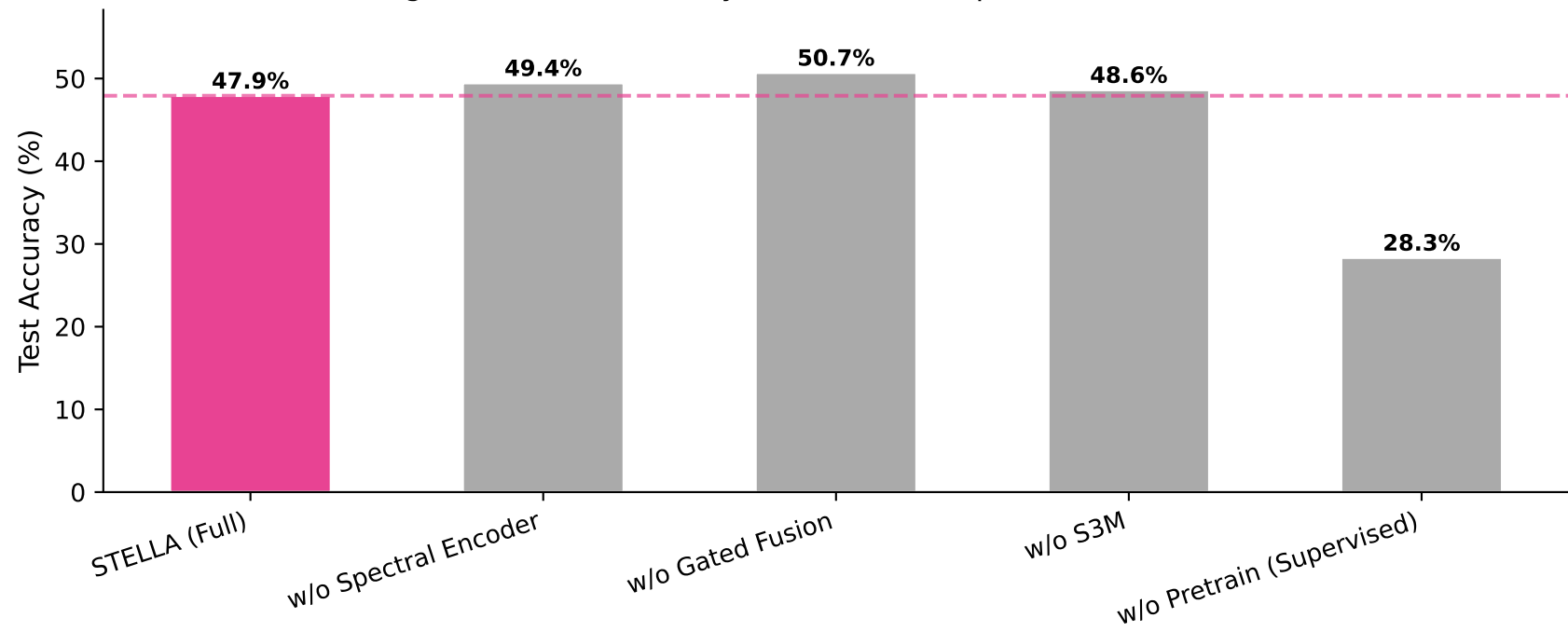
Figure 7: Ablation Study — STELLA Component Contributions
