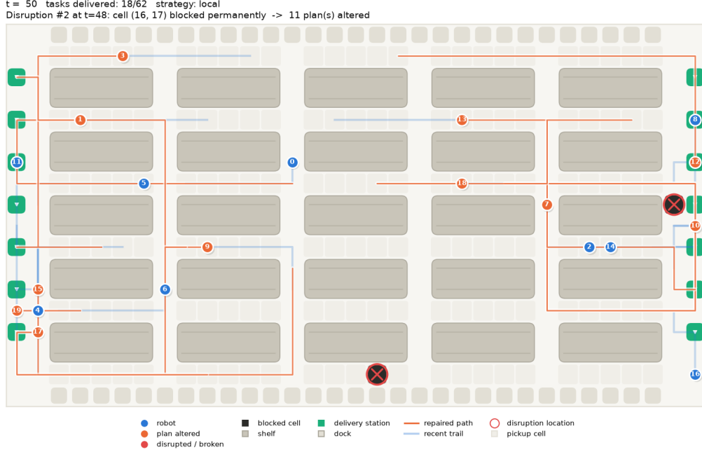
Figure 10: A frame from the demonstration video, two steps after a permanent blockage (red circle) that changed 11 plans. Orange robots have altered plans; orange lines are their repaired paths.
