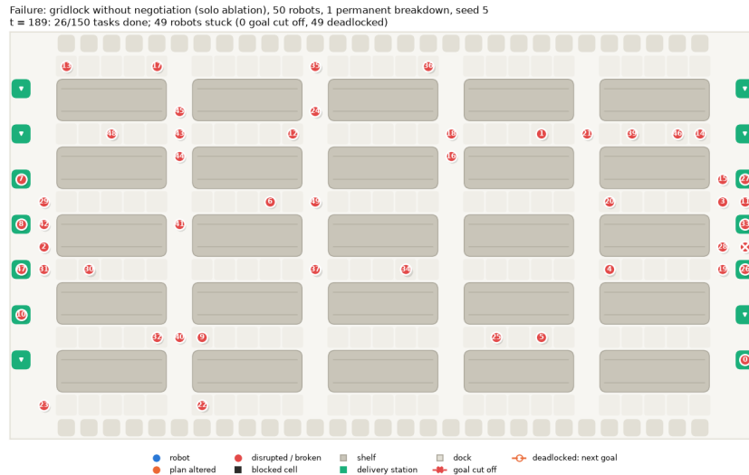
Figure 9: Gridlock without negotiation ( solo ): after one permanent breakdown all 49 remaining robots (red) wait on each other. Our method completes all 150 tasks on the same instance.
