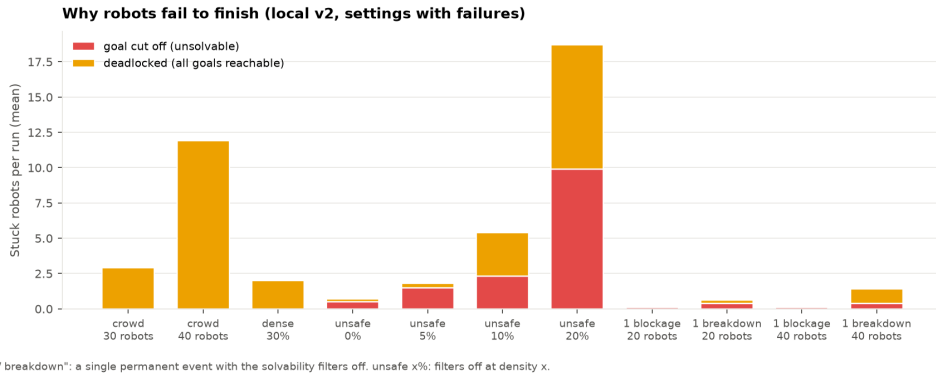
Figure 7: Why robots fail to finish under our method: goal cut off (red) or deadlocked although every goal is reachable (orange).
