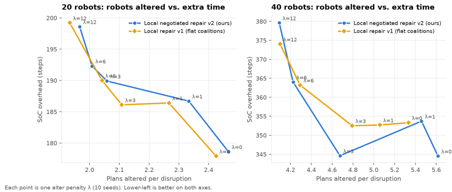
Figure 5: Plans changed vs. extra time as the alter penalty \lambda varies (ours vs. our first version).
