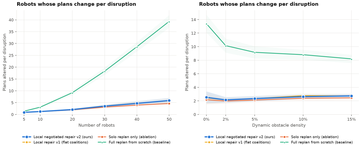
Figure 2: Plans changed per disruption vs. number of robots (left) and dynamic obstacle density (right, 20 robots). Bands are 95% confidence intervals.
