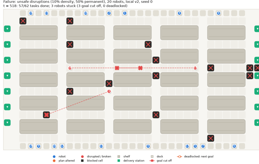
Figure 8: A failure from the demonstration: permanent blockages (black) cut off the goals of robots 3, 13 and 18, and 5 of 62 tasks are never done.
