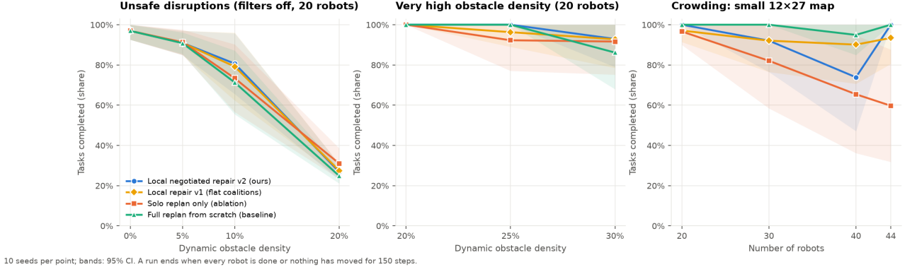
Figure 6: Share of tasks completed in the stress settings (10 seeds per point).
