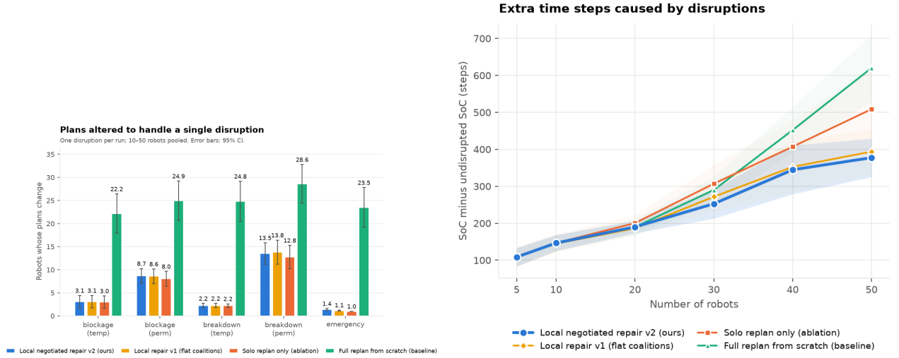
Figure 4: Left: plans changed to handle a single disruption, by type (10–50 robots pooled). Right: extra time steps caused by disruptions vs. number of robots.
