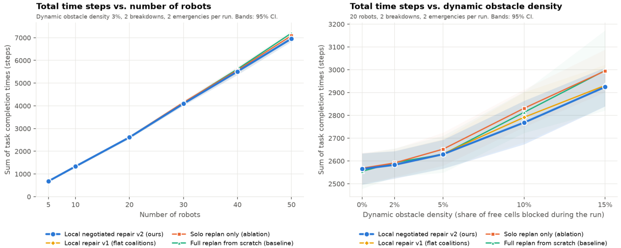
Figure 3: Total time steps (SoC) vs. number of robots (left) and vs. dynamic obstacle density (right, 20 robots). Bands are 95% confidence intervals.
