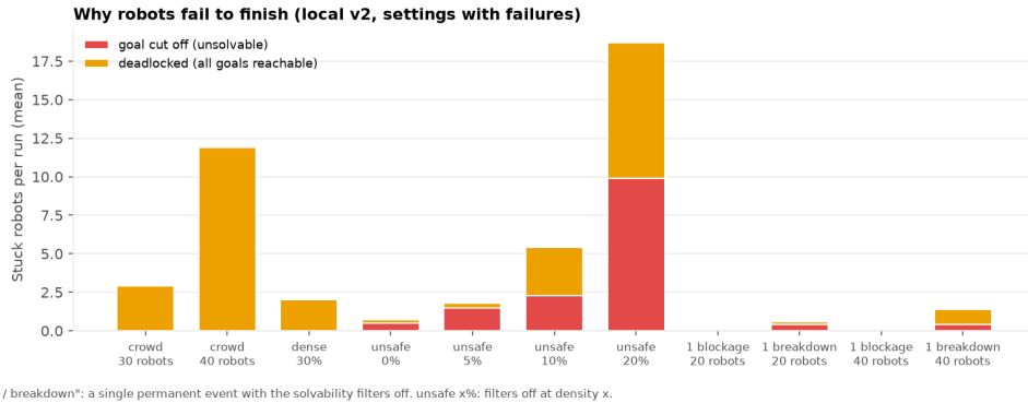
Figure 7: Why robots fail to finish under our method: goal cut off (red) or deadlocked although every goal is reachable (orange).
