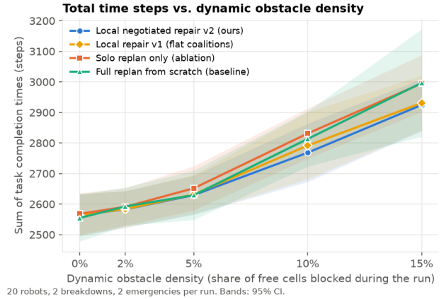
Figure 3: Total time steps (SoC) vs. number of robots (left) and vs. dynamic obstacle density (right, 20 robots). Bands are 95% confidence intervals.
