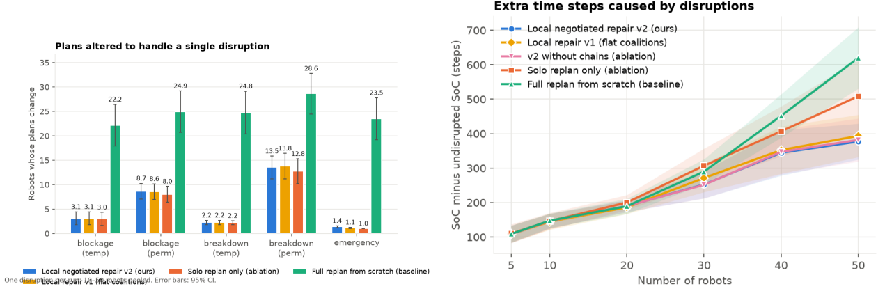
Figure 4: Left: plans changed to handle a single disruption, by type (10–50 robots pooled). Right: extra time steps caused by disruptions vs. number of robots.
