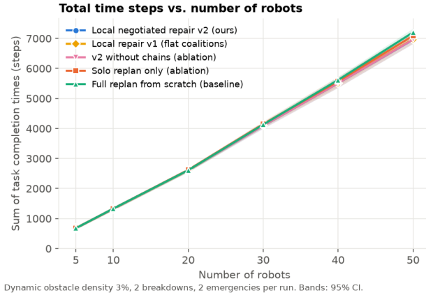
Figure 3: Total time steps (SoC) vs. number of robots (left) and vs. dynamic obstacle density (right, 20 robots). Bands are 95% confidence intervals.
