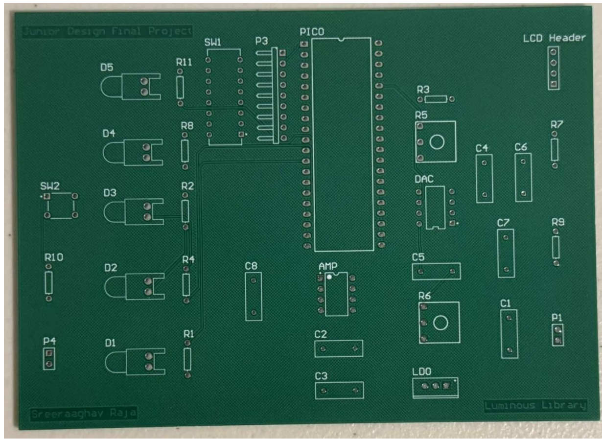
Figure 12: Empty PCB
