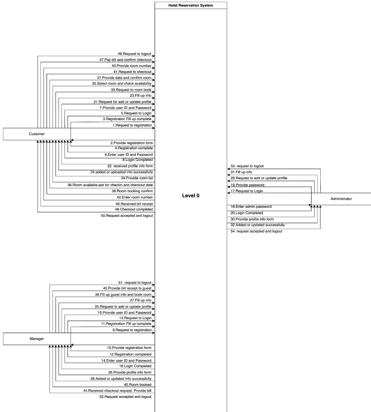
Figure: Data Flow Diagram level 0
