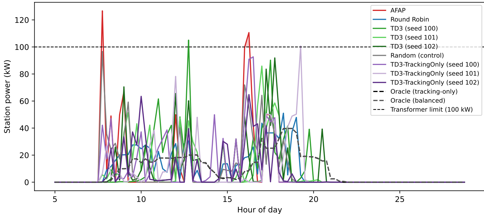
Aggregate station power, reference day 2022-01-17 (station_v0 bogota, seed=0)
