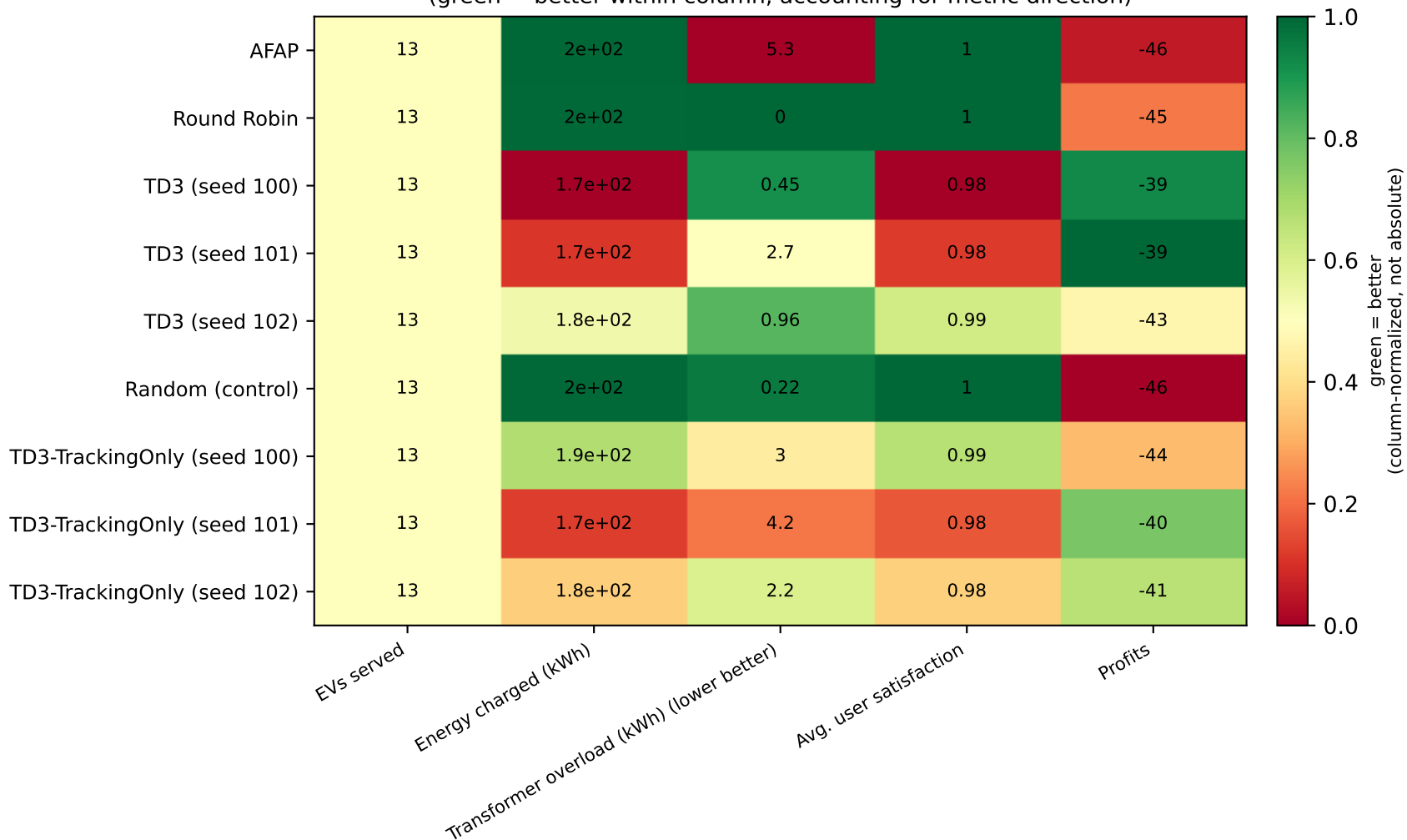
station_v0_bogota: algorithm x metric summary (green = better within column, accounting for metric direction)
