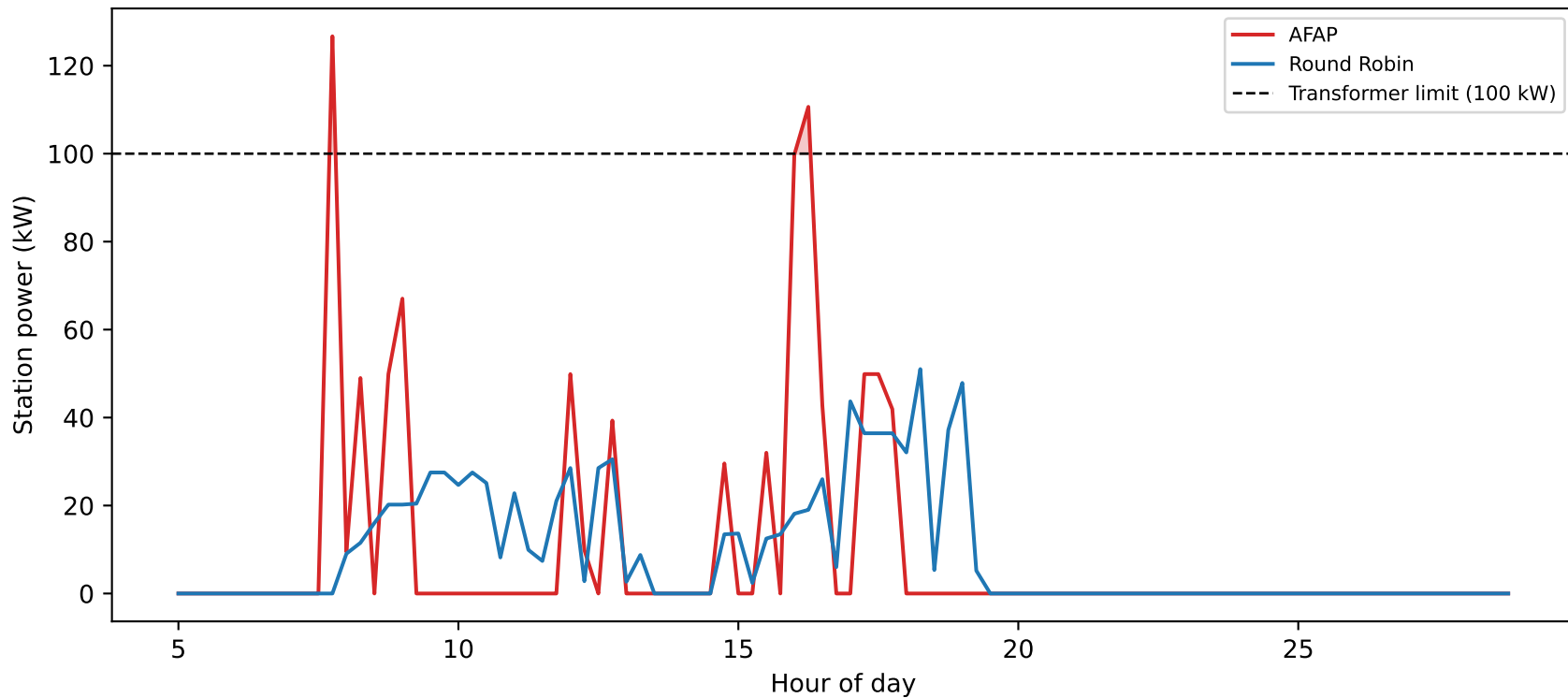
Aggregate station power, reference day 2022-01-17 (station_v0_bogota, seed=0)
