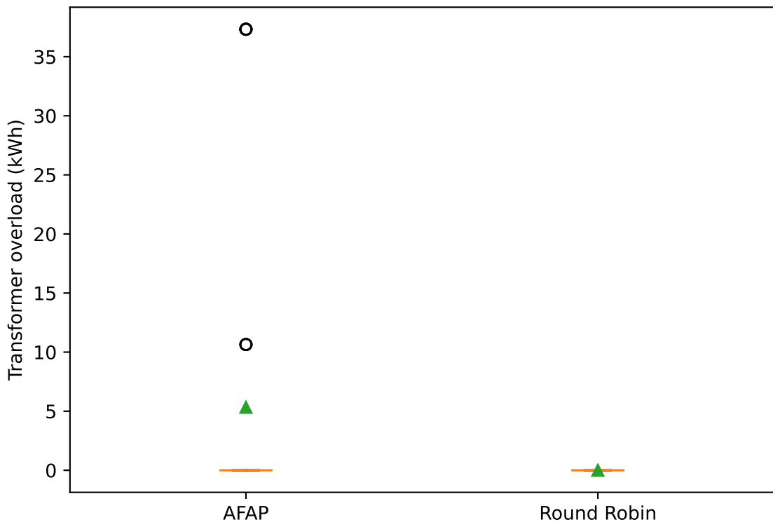
station_v0_bogota: Transformer overload (kWh) distribution across all 50 runs per algorithm (5 seeds x 10 days)
