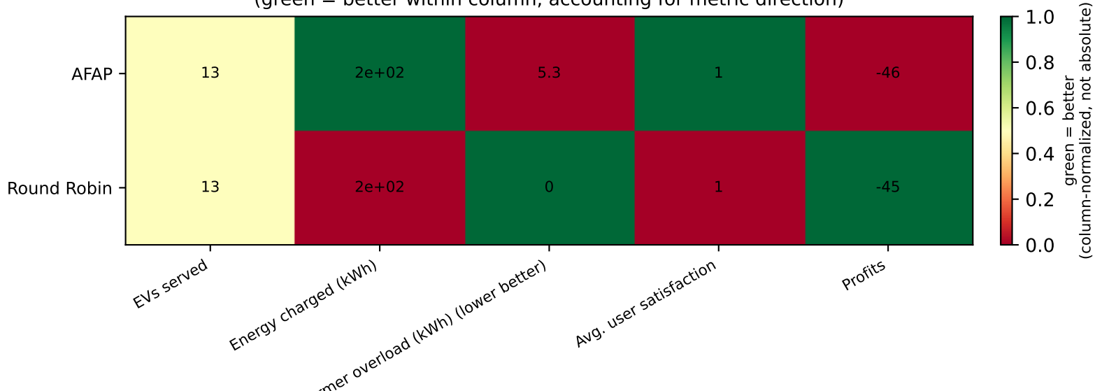
station_v0_bogota: algorithm x metric summary (green = better within column, accounting for metric direction)
