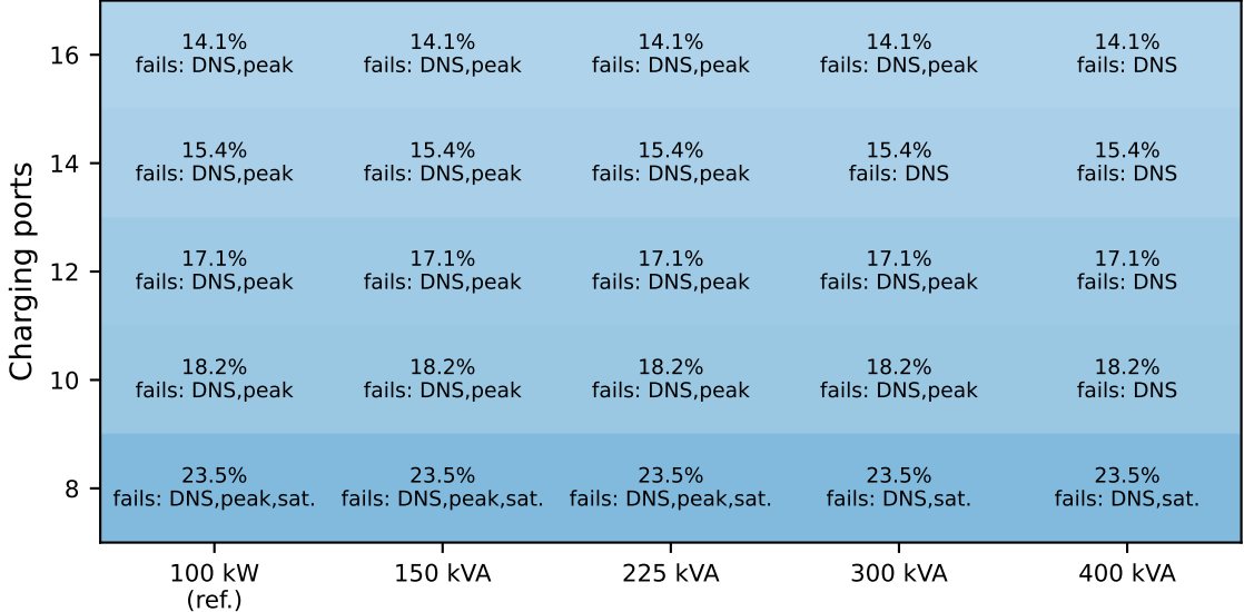
Round Robin, transformer-aware, 1.3x
