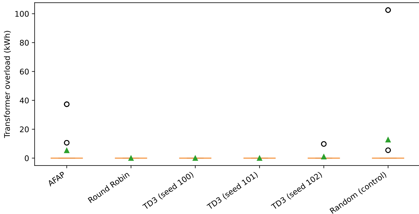
station_v0_bogota: Transformer overload (kWh) distribution across all 50 runs per algorithm (5 seeds x 10 days)
