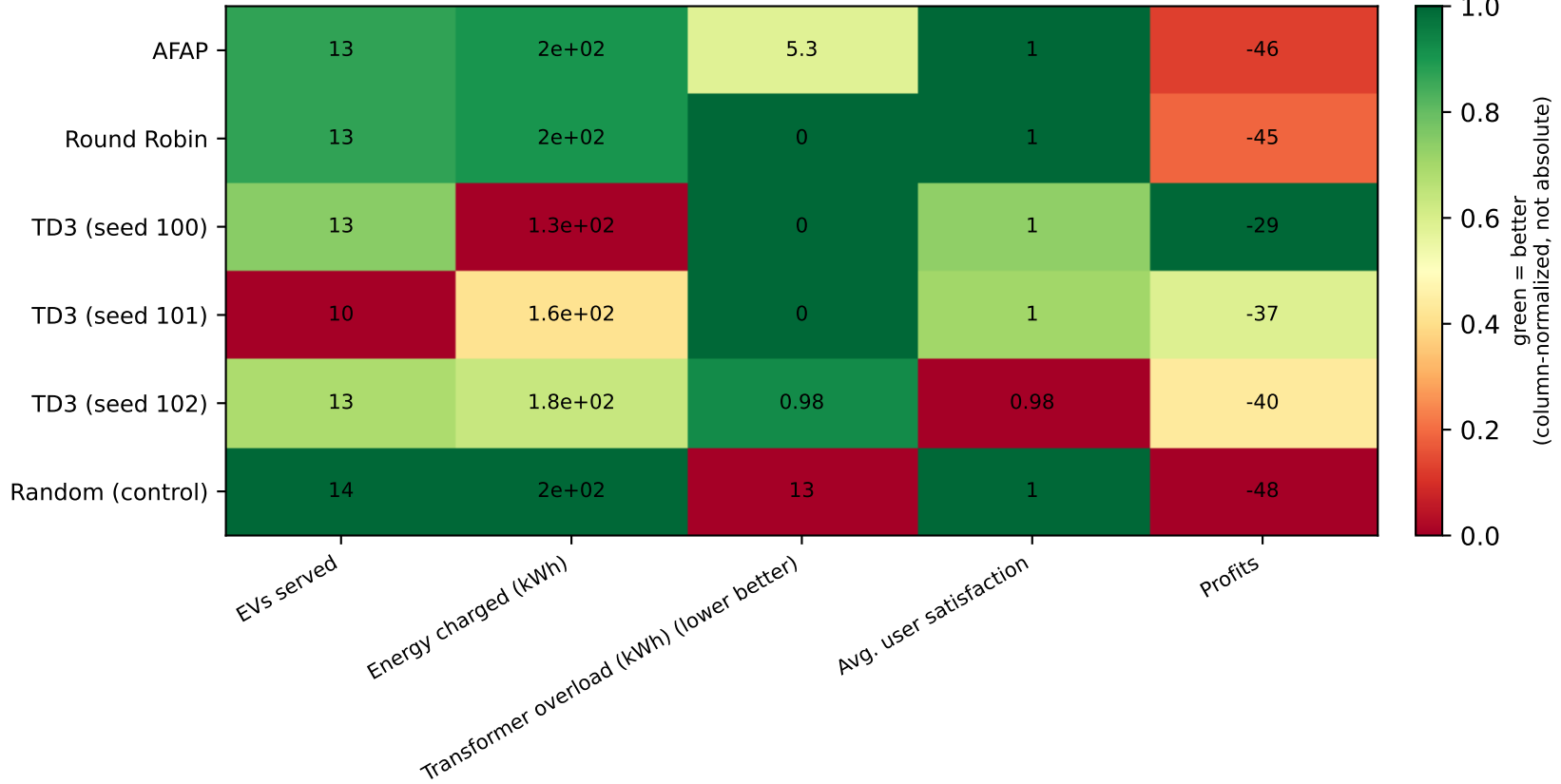
station_v0_bogota: algorithm x metric summary (green = better within column, accounting for metric direction)
