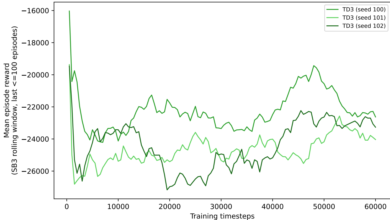
TD3 vanilla learning curves, one line per training seed (station_v0_bogota, TRAIN_DAYS round-robin)
