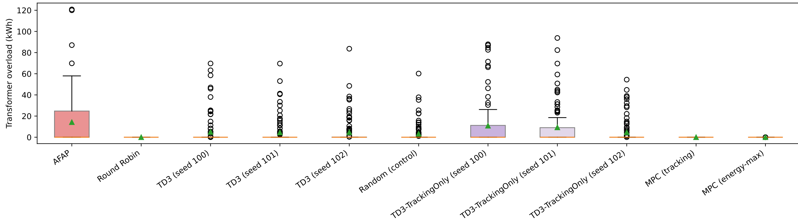
station_v0_bogota: Transformer overload (kWh) distribution across all 100 runs per algorithm (50 seeds x 2 day types)
