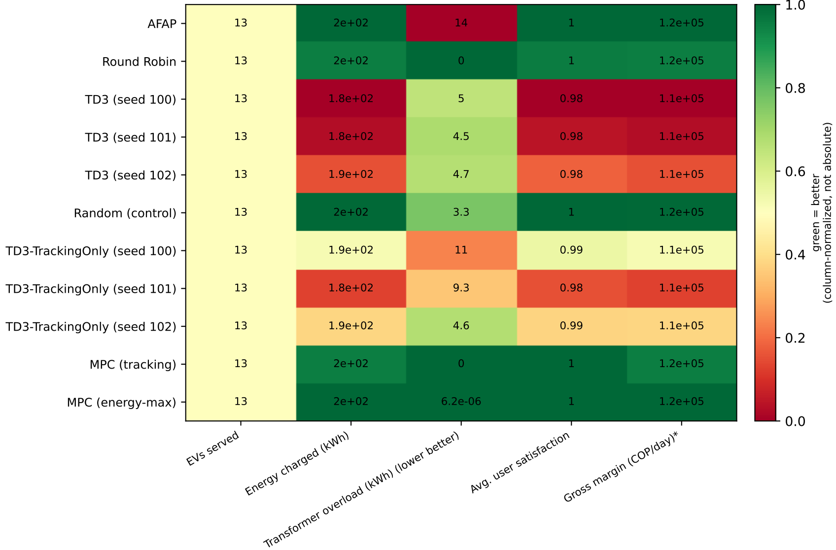
station_v0_bogota: algorithm x metric summary (green = better within column, accounting for metric direction)
