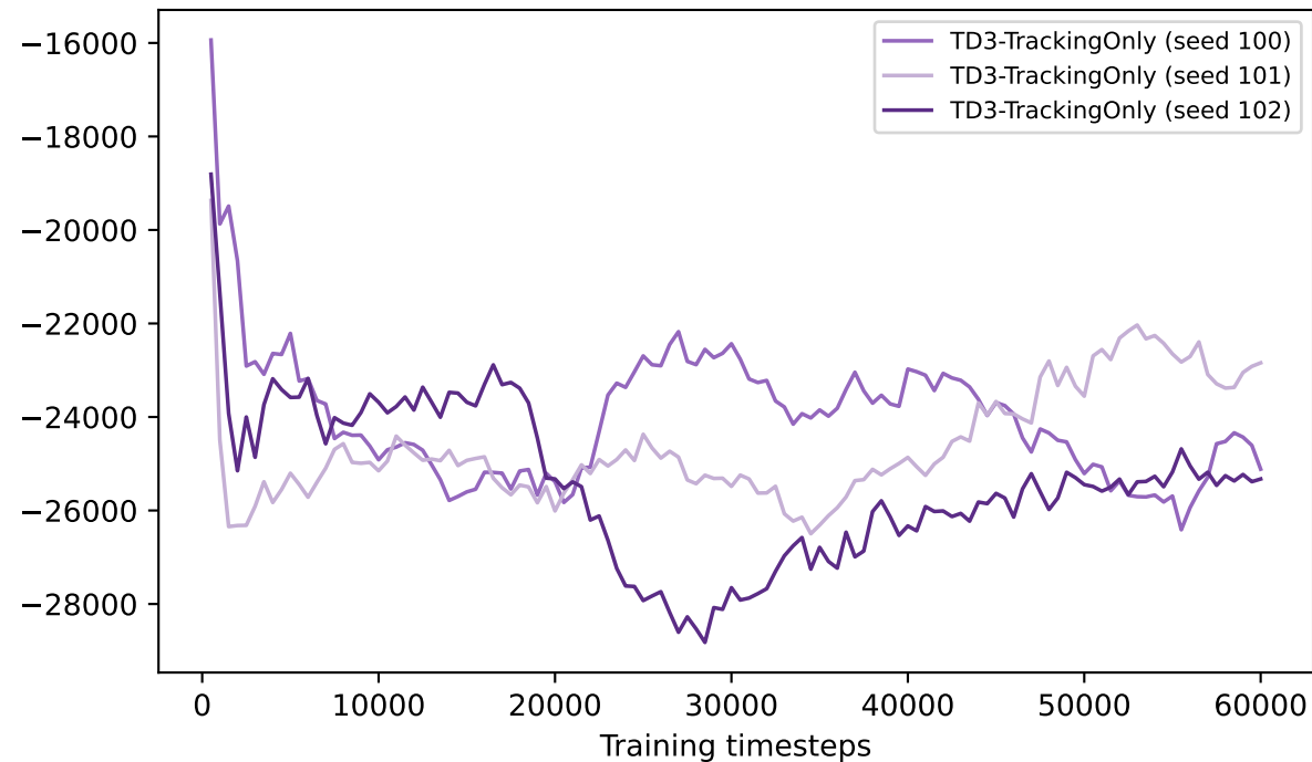
TD3-TrackingOnly
