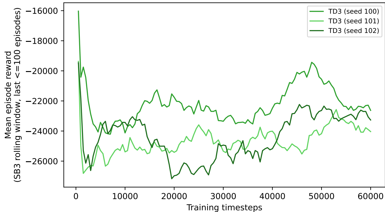
TD3 vanilla
