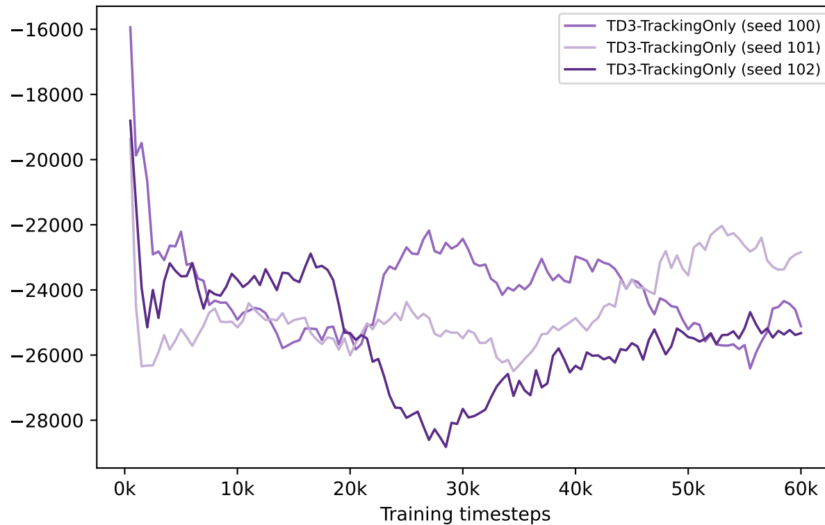
TD3-TrackingOnly (original runs, 60k steps)
