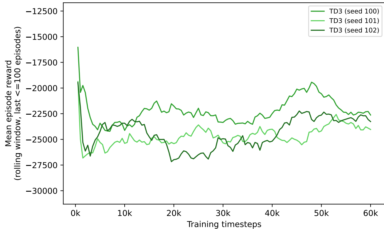
TD3 vanilla (original runs, 60k steps)
