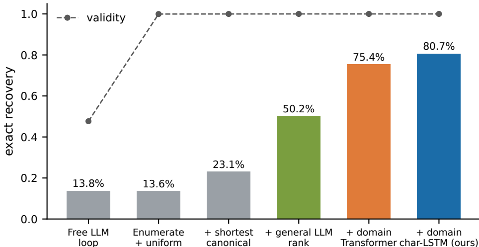
Figure 3: Exact recovery (bars) and validity (dashed) as the free-generation loop is replaced by enumeration and progressively better selection rules.
