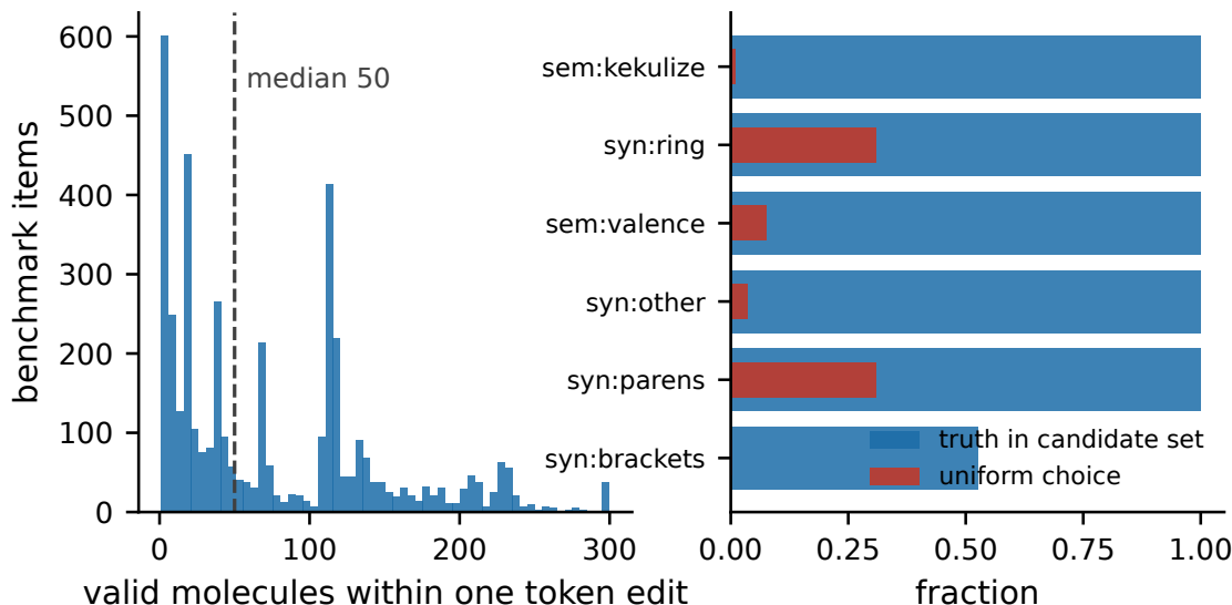
Figure 2: Left: number of valid molecules within one token edit. Right: per error category, the fraction of items whose candidate set contains the truth (blue) and the expected accuracy of uniform selection (red).
