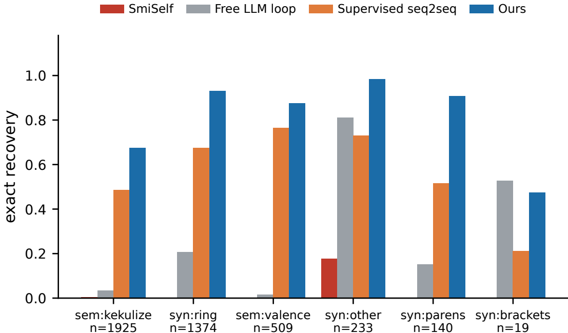
Figure 4: Exact recovery by error category.
