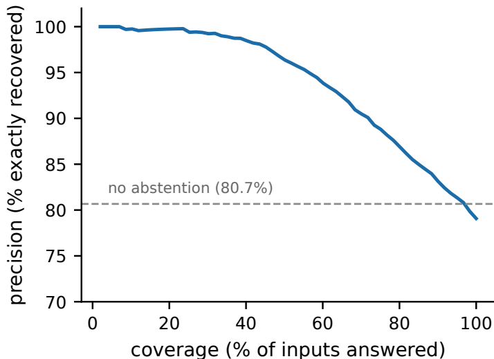
Figure 5: Risk-coverage curve for ENUMRANK, over the 3,881 test items for which the ranking margin is defined. Answering the most confident half of them (46% of the full test split) gives 96.4% precision.
