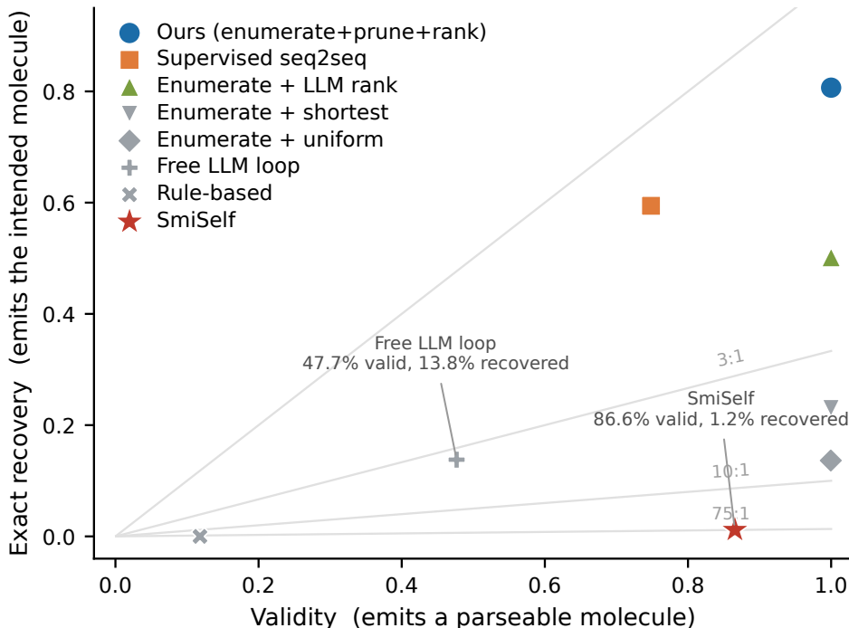
Figure 1: Validity and recovery are close to independent. Grey lines are contours of constant valid-outputs-per-correct-recovery. Two systems are annotated whose relative ordering depends entirely on which axis is read.
