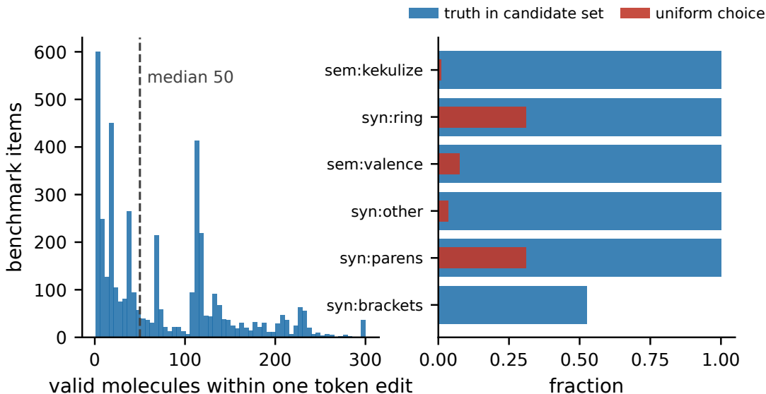
Fig. 2: Left: number of valid molecules within one token edit. Right: per error category, the fraction of items whose candidate set contains the truth (blue) and the expected accuracy of uniform selection (red).
