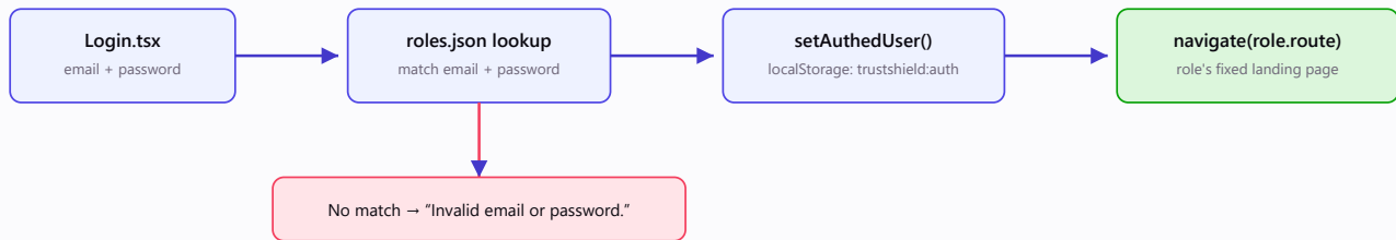
Fig. 1 — Authentication & role routing flow (Login.tsx → auth.ts → role landing route)
