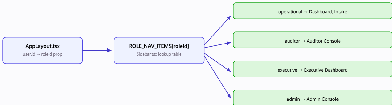
Fig. 2 — Sidebar navigation resolved per role via ROLE_NAV_ITEMS lookup ( Sidebar.tsx )
