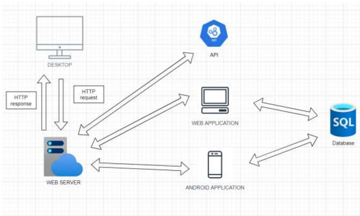
Figure 41 Software Architecture
