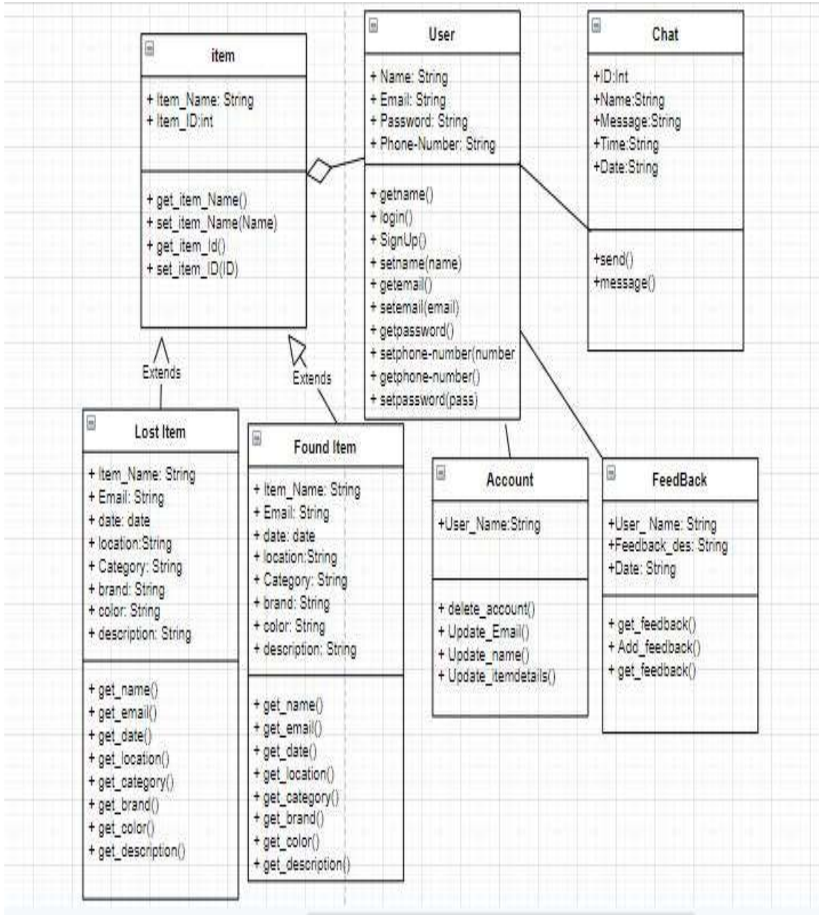
Figure 42 Class diagram
