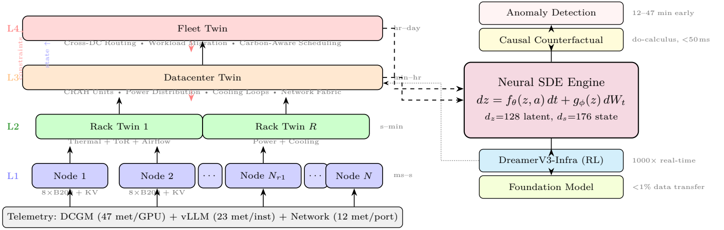
Fig. 1. InferTwin system architecture. Left: Four-level hierarchical digital twin (L1–L4) mirrors the physical datacenter—state aggregates upward while constraints propagate downward at each level’s natural timescale. Right: Neural SDE engine ( d_z=128 latent, d_s=176 state) powers four applications: anomaly detection (12–47 min early warning), causal counterfactual queries (<50 ms), DreamerV3-Infra offline RL (1000 \times real-time training), and cross-facility foundation model transfer.
