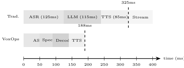
Fig. 4. Speculative prefill pipeline. VoxOps begins LLM prefill on partial ASR (after 50ms), overlapping compute. First audio output at 188ms vs. 325ms traditional.
