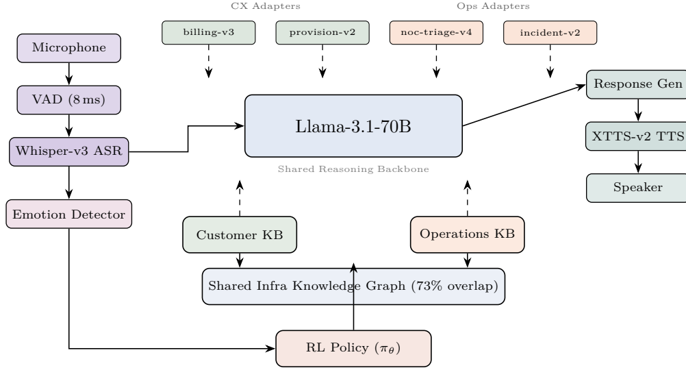
Fig. 1. VoxOps unified architecture. A single LLM backbone serves both CX and Ops via hot-swappable LoRA adapters. The shared knowledge graph (73% overlap) enables cross-domain context. Emotion detection feeds the RL policy. Pipeline achieves 188 ms P50 latency.
