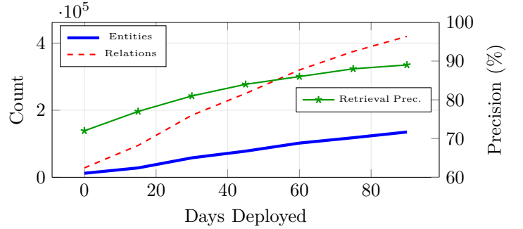
Fig. 6. Knowledge graph growth dynamics over 90-day deployment. Entity and relation counts grow linearly while retrieval precision improves logarithmically, indicating compounding returns from accumulated knowledge.
