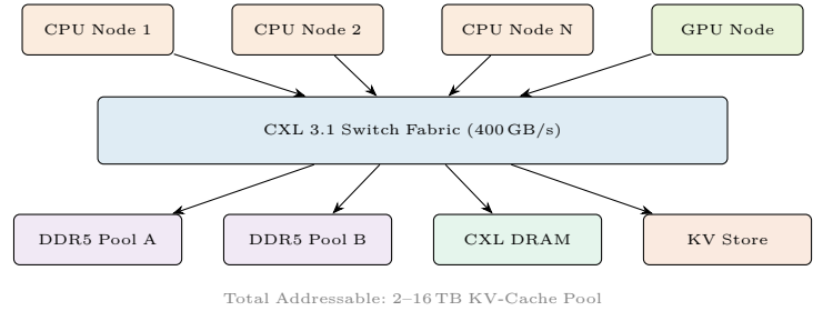
Fig. 2. CXL 3.1 memory pooling for disaggregated KV-cache. Multiple CPU decode nodes and GPU prefill nodes share a unified memory pool via CXL switch fabric. Any node can access any KV-cache page with <300 ns additional latency vs. local DRAM.
