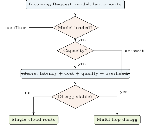
Fig. 8. Multi-objective routing decision framework. Each request is scored across latency, cost, quality, and overhead dimensions before selecting single-cloud or disaggregated multi-hop routing.
