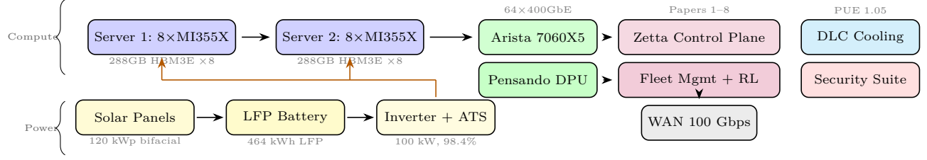
Fig. 1. SolarInfer Edge SKU complete architecture. Power tier (solar + BESS) feeds compute tier (2x8-GPU servers), connected via 400GbE fabric with DPU-based telemetry to the Zetta control plane. DLC cooling maintains PUE of 1.05.
